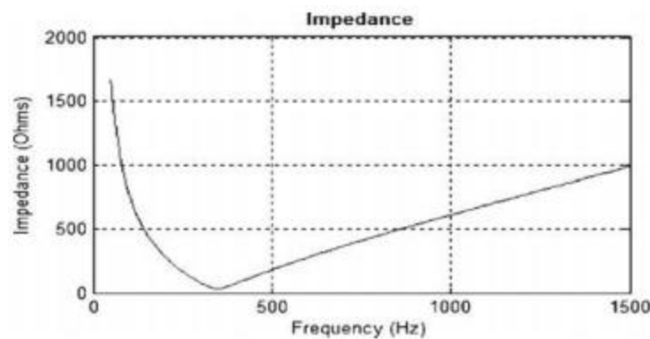
Figure 4.2: impedance vs frequency curve [38]
