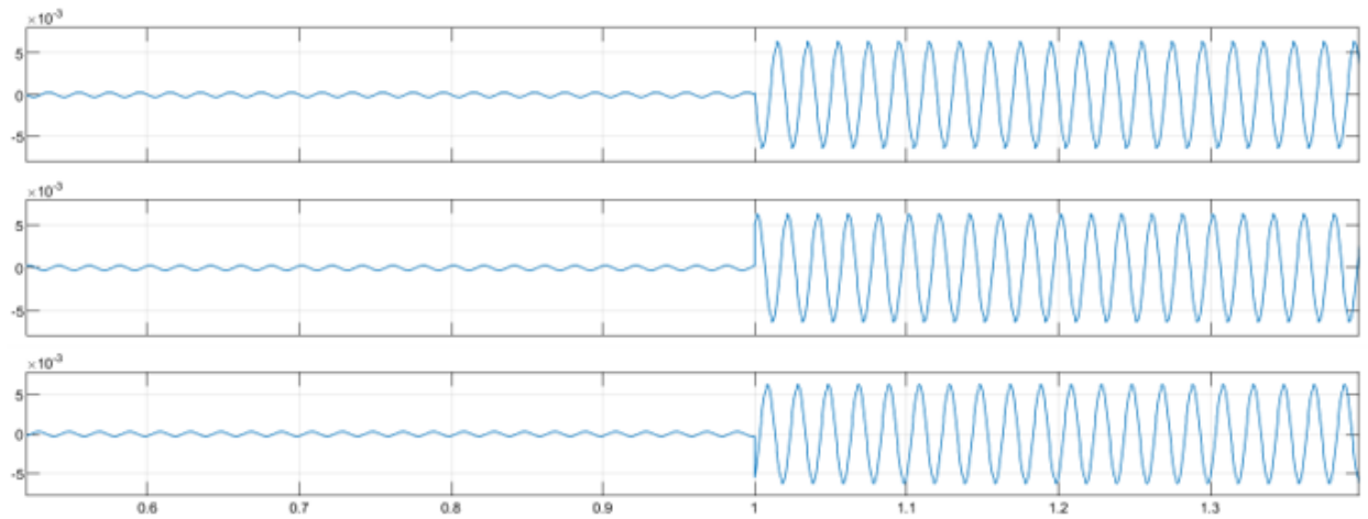
Figure 5.10: Filter current without Compensation
