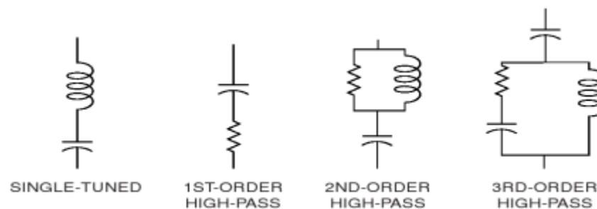
Figure 4.1: schematic diagram of series tuned filter [38]
