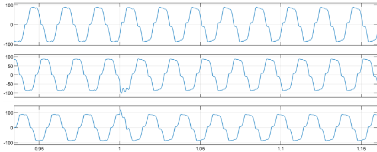
Figure 5.7: Three-phase source current with nonlinear load
