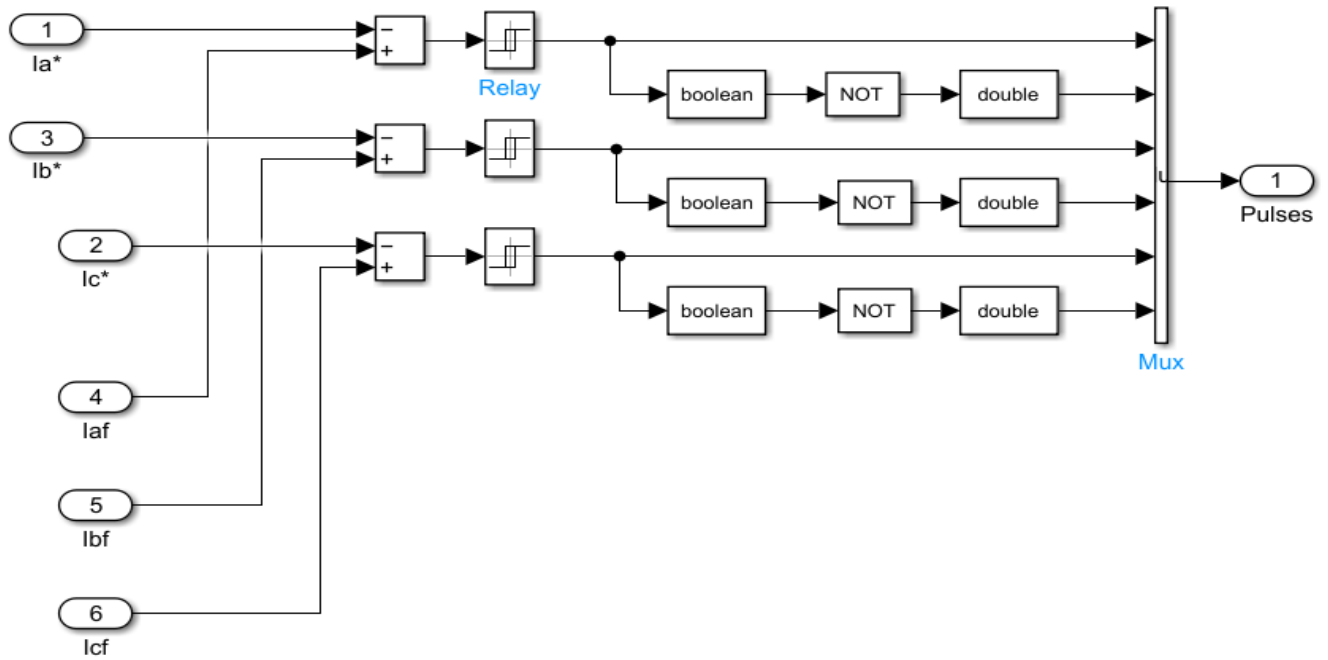
Figure 5.5: Hysteresis Current regulator
