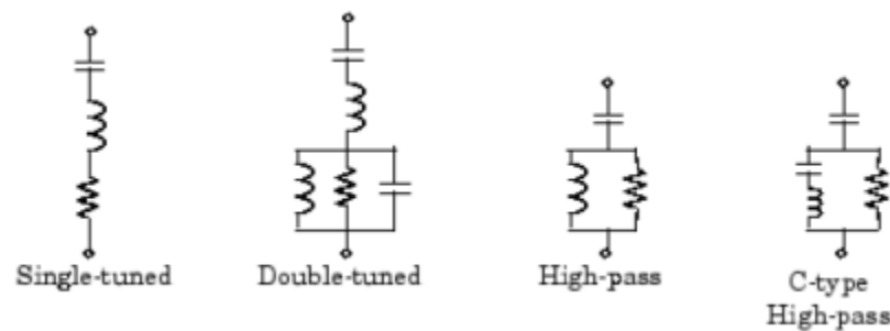
Figure 3.2: Different types of three-phase RLC harmonic filter [34]
