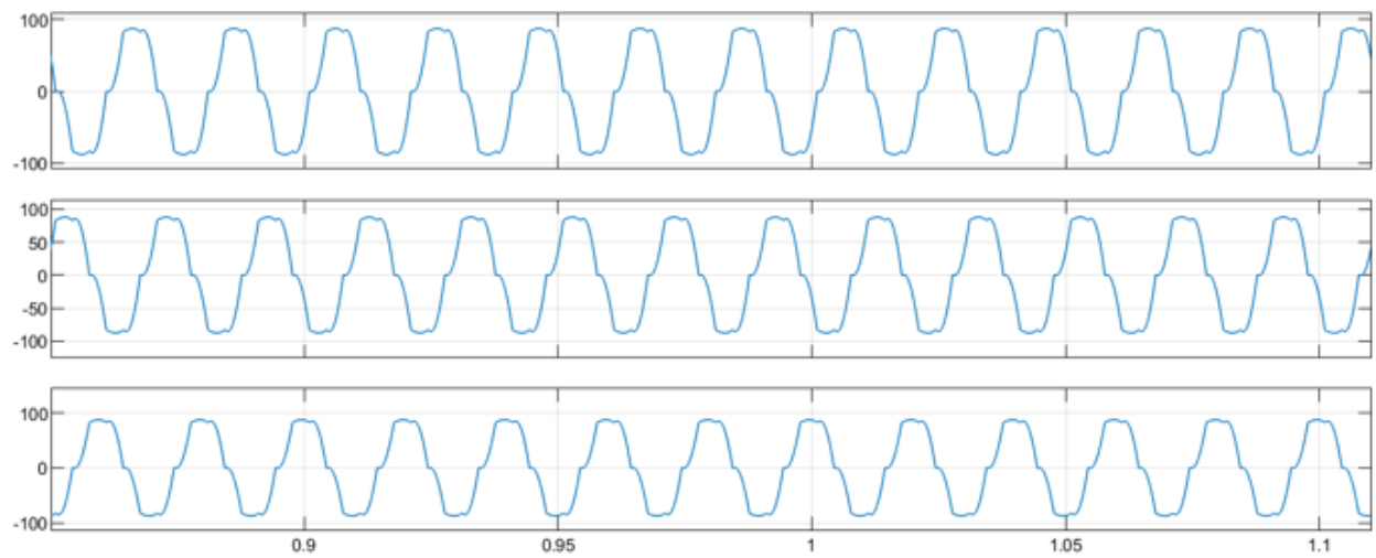
Figure 5.9: Source current without compensation
