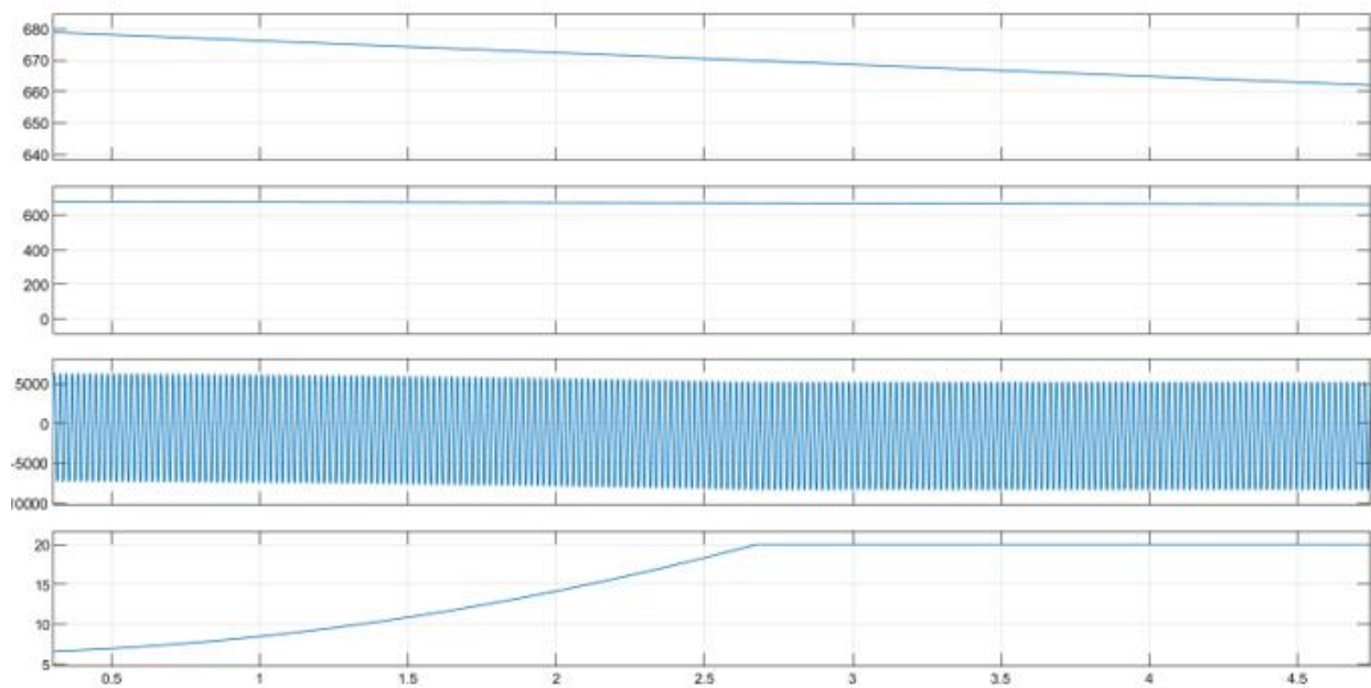
Figure 5.11: Three-phase compensated Current and Voltage
