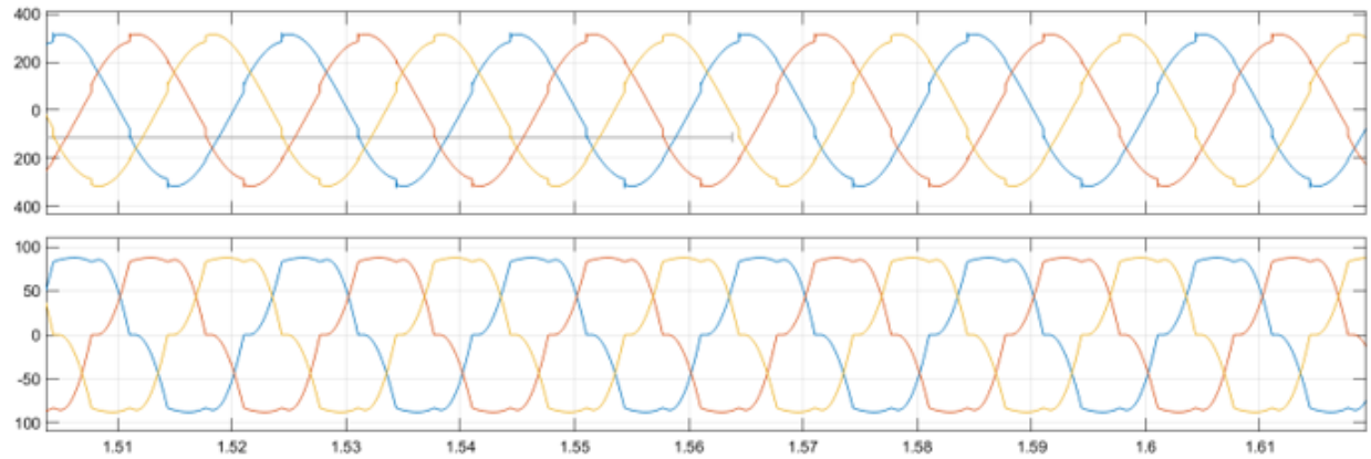
Figure 5.12: Three- phase compensation load current
