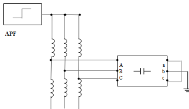
Figure 5.3: LCL filter
