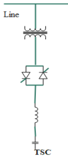
Figure 1.12: General structure of TSC
